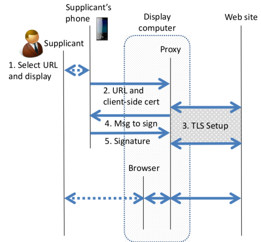
Fig. 3. Use of DNo to establish TLS connection.
