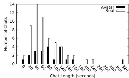
Fig. 7. Histogram of chat lengths, binned into 20-second intervals.
