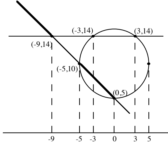
Figure 3: Equivalent points and formula satisfaction.
