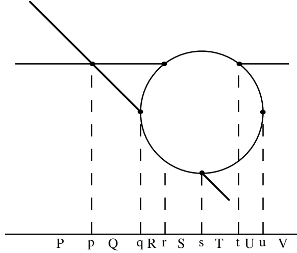
Figure 2: From equivalence classes in A^2 (Example 2.5) to equivalence classes in A .
