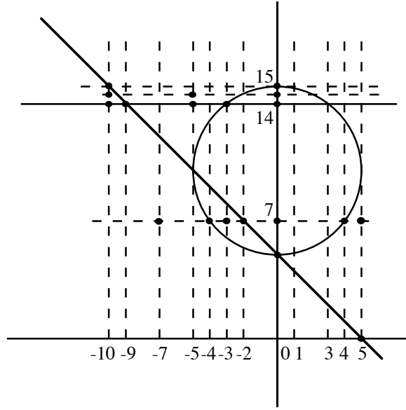
Figure 4: Domain sequence construction.
