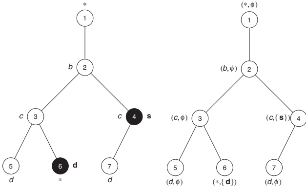
FIGURE 16. A tree query and its encoding as a labeled tree.
