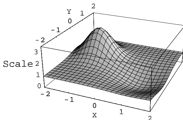
Figure 4: A scaling field that could be used, in regions of value greater than unity, to magnify the screen distance traversed by a unit mouse motion; similarly, in regions of value less than unit, this field would slow the mouse response to provide extremely fine-grained control in those limited areas where it is required.
