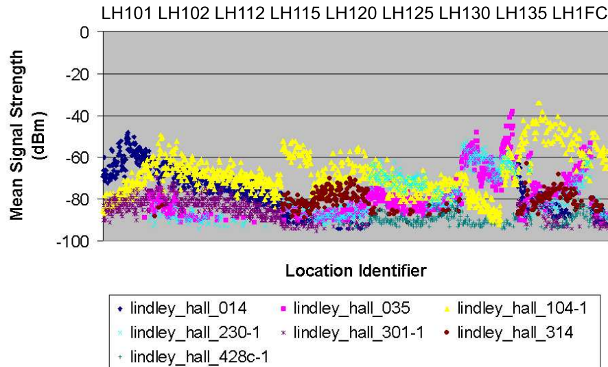
Figure 1: Processed signal strength by location identifier. It can be observed graphically unique patterns of AP signal strength exist.
