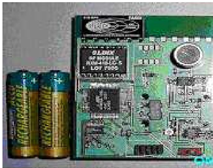
Figure 10: Figure of Cricket Listener
