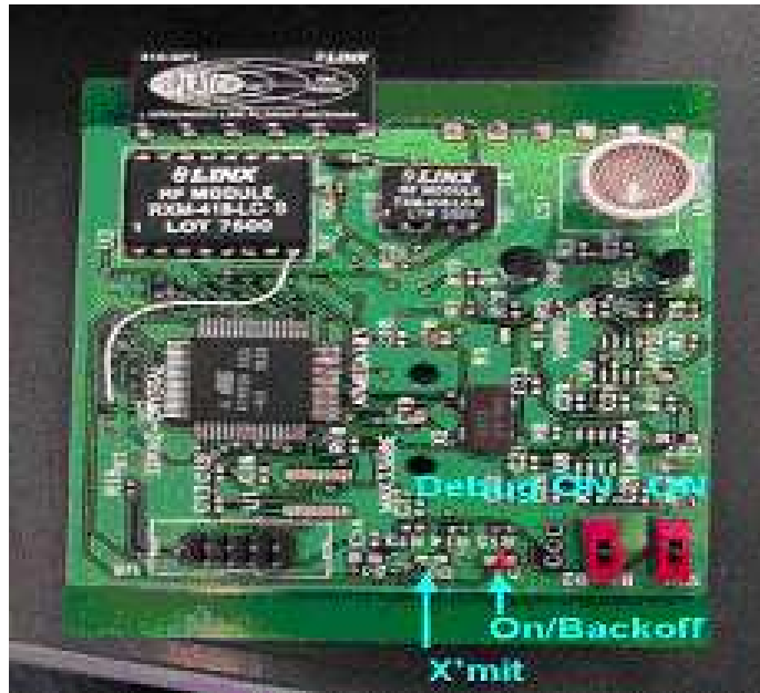
Figure 9: Figure of Cricket Beacon
