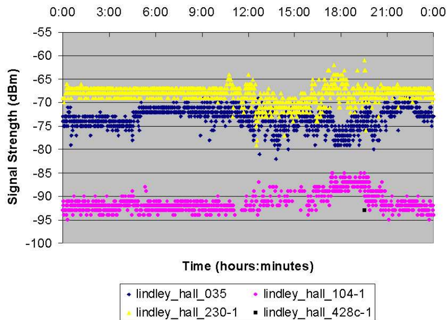
Figure 2: 24 hour analysis of signal strengths
