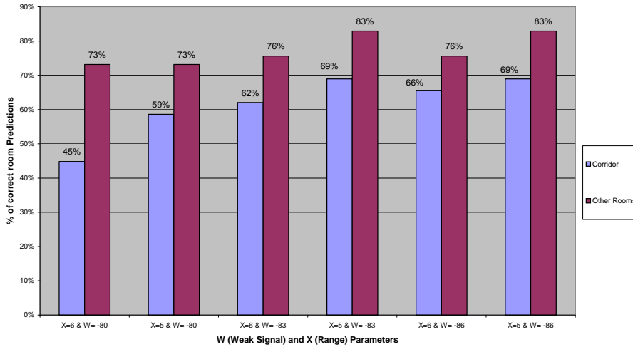
Figure 5: Performance of corridor Vs rooms
