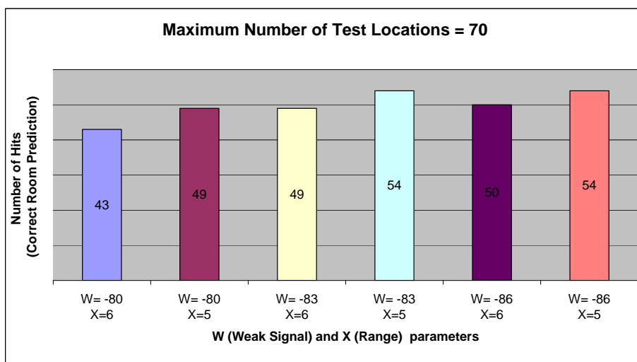
Figure 3: Analysis of prediction of correct rooms
