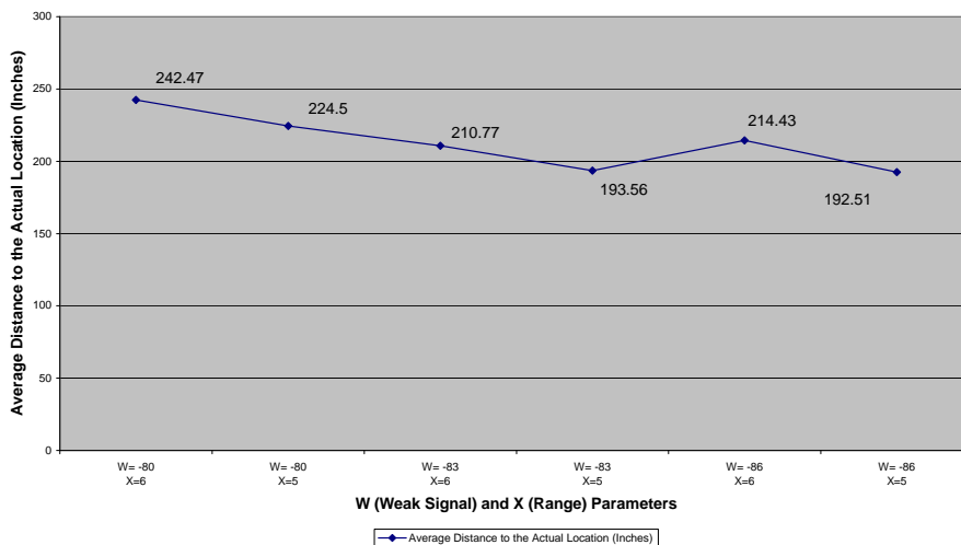
Figure 4: Analysis of average distance between the predicted and actual location
