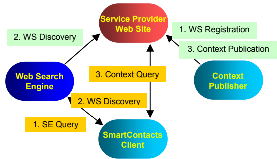
Figure 2. SmartContacts workflow
