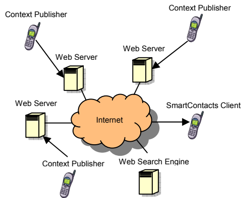
Figure 1. Overview of SmartContacts
