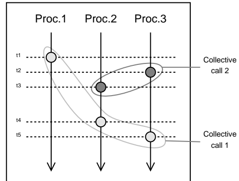
Figure 5. The synchronization problem: if the PRMI call is delivered as soon as one process reaches the calling point, the remote component will block at t_1 waiting for data from processes 2 and 3, and will not accept the second collective call at t_2 and t_3 . The remote component will be blocked indefinitely because processes 2 and 3 will never reach t_4 and t_5 to complete the first call. The solution is to delay PRMI delivery until all processes are ready.
