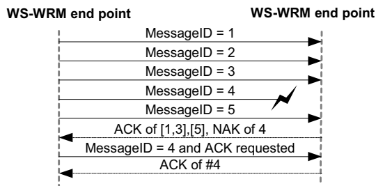
Figure 4. Guaranteed Message Deliveries in WS-WRM scheme
