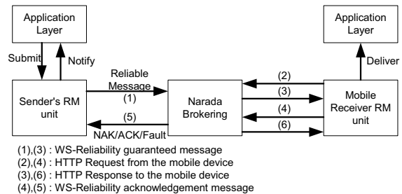
Figure 3. Example of HTTP binding to implement a guaranteed message delivery with WS-Reliability in mobile environments
