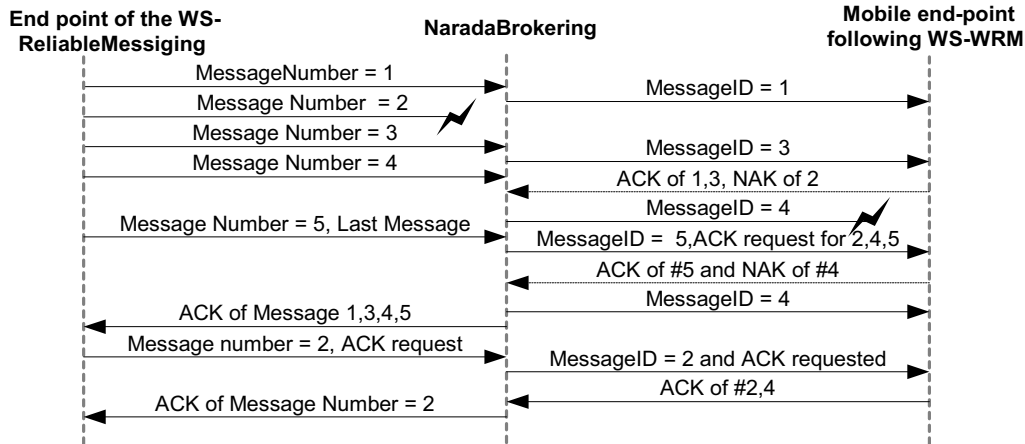
Figure 8. Example of cooperating WS-WRM and WS-ReliableMessaging
