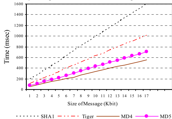
Figure 6. Generating message digest on Smartphone (Treo300)
