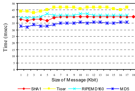
Figure 7. Comparison of message digests on Smartphone (Treo300)
