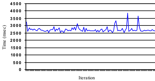
Figure 1. Performance of HTTP connection with the wireless telephone network (data size: 1Kb, J2ME platform, Treo 300)
