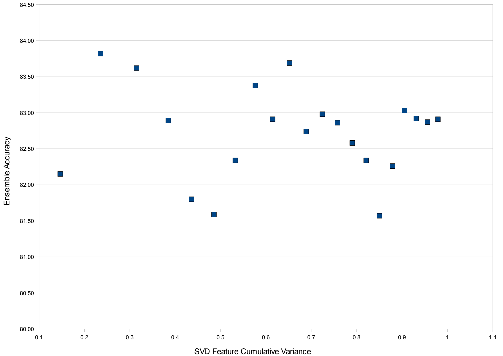
Heart - Accuracy vs. SVD Cumulative Variance
