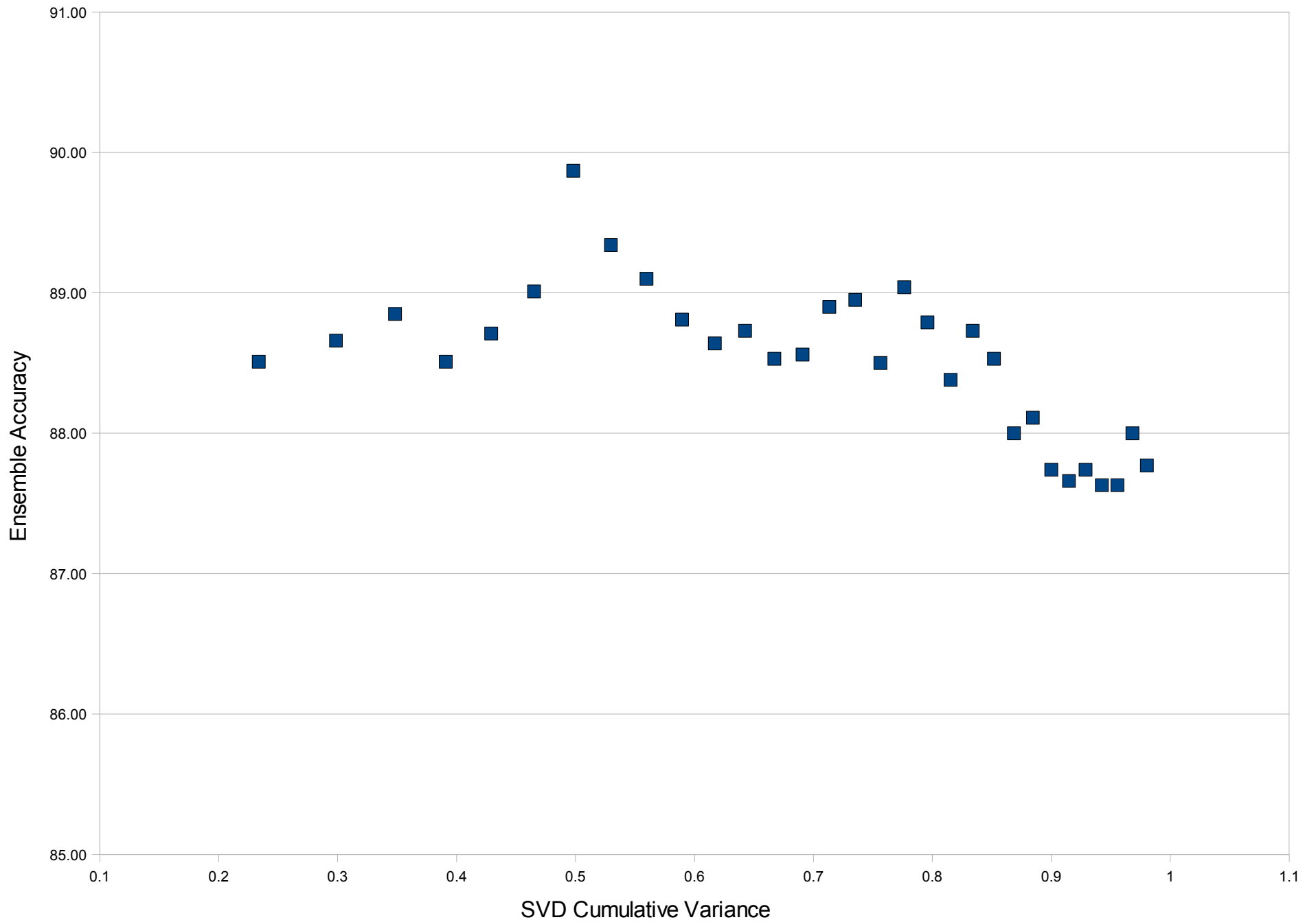
Ionosphere - Accuracy vs. SVD Cumulative Variance
