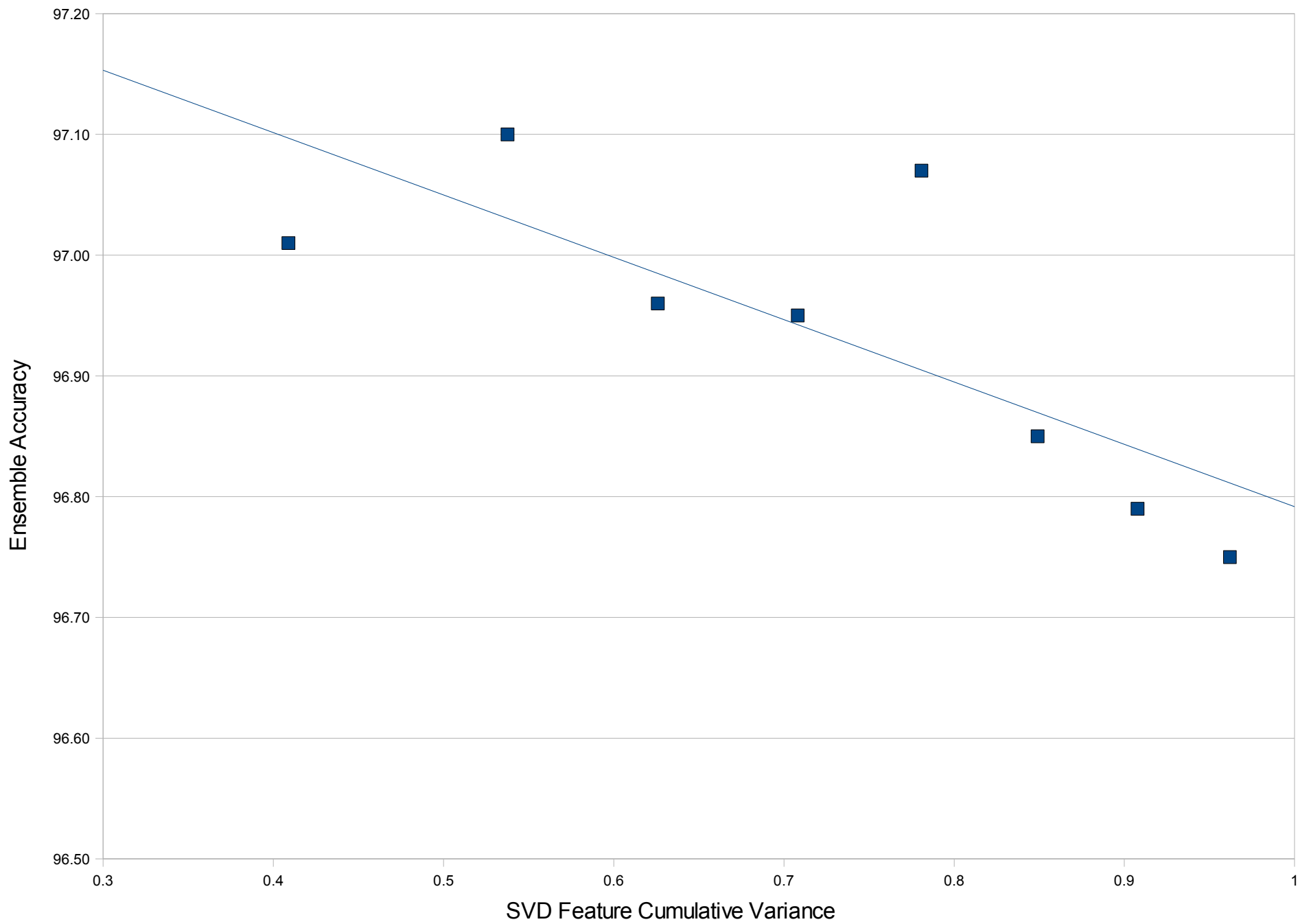
Breast Cancer - Accuracy vs. SVD Cumulative Variance
