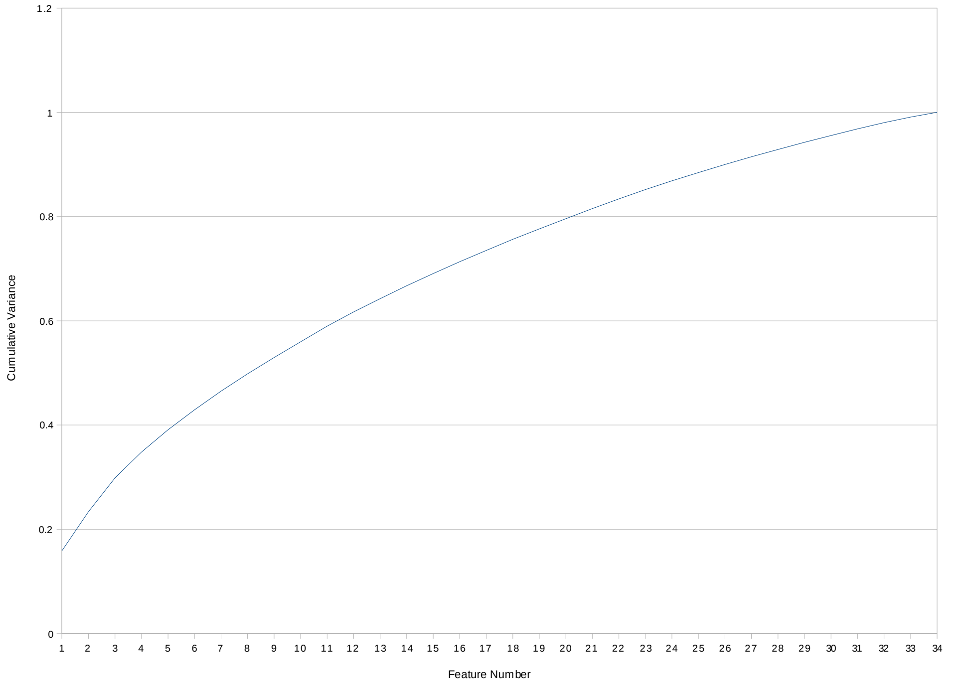
Ionosphere SVD Feature Cumulative Variance
