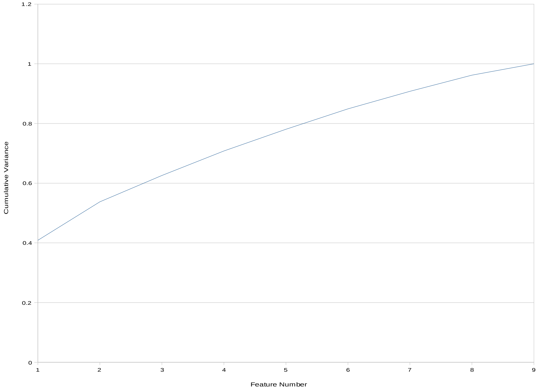
Breast Cancer SVD Feature Cumulative Variance
