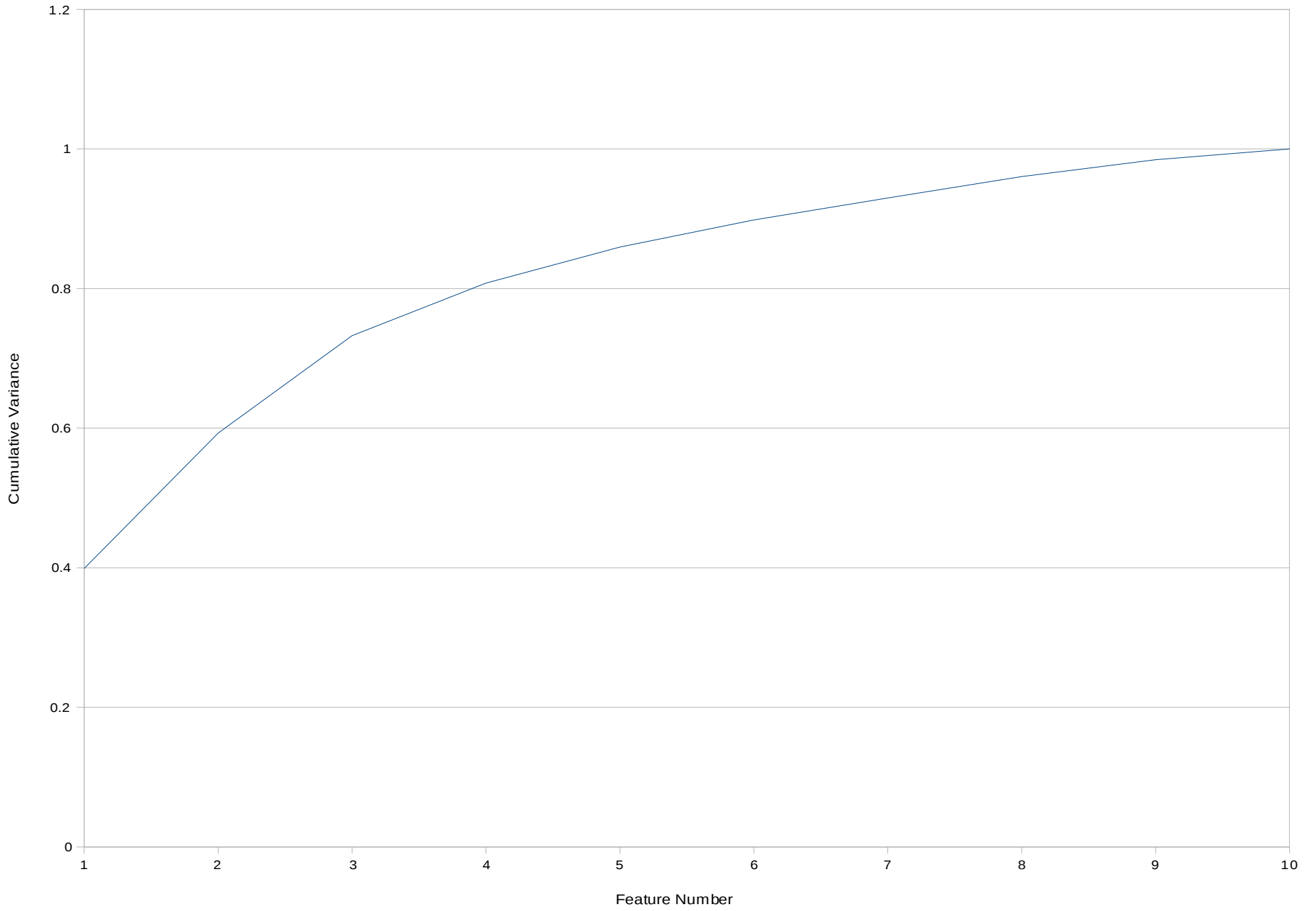
Telescope SVD Feature Cumulative Variance
