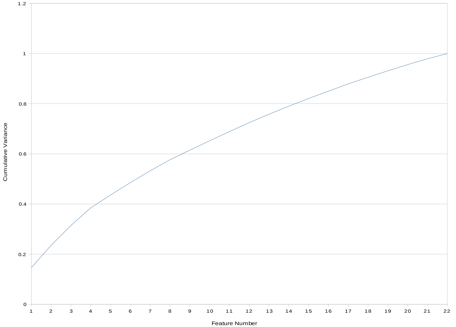
Heart SVD Feature Cumulative Variance
