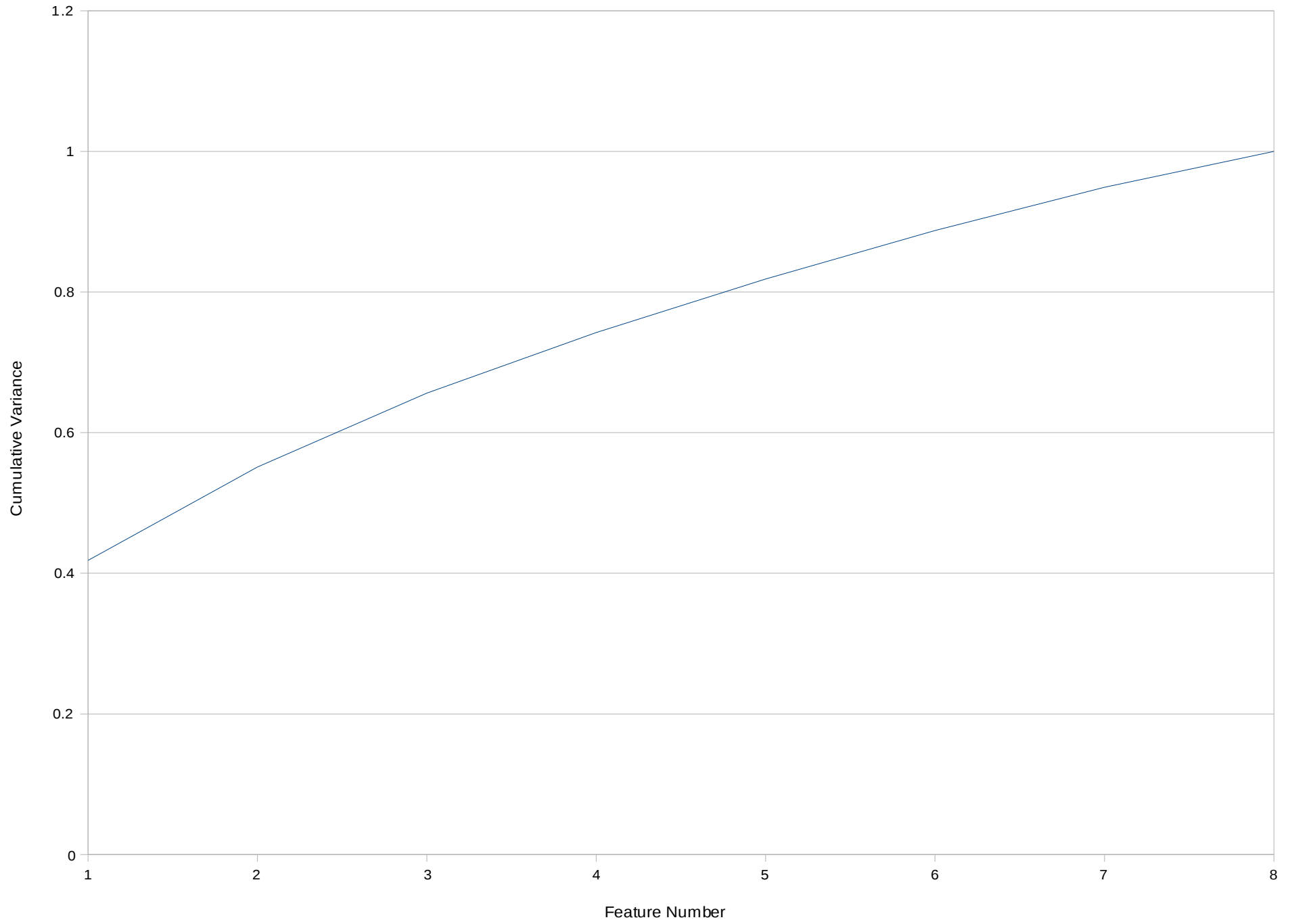
Diabetes SVD Feature Cumulative Variance
