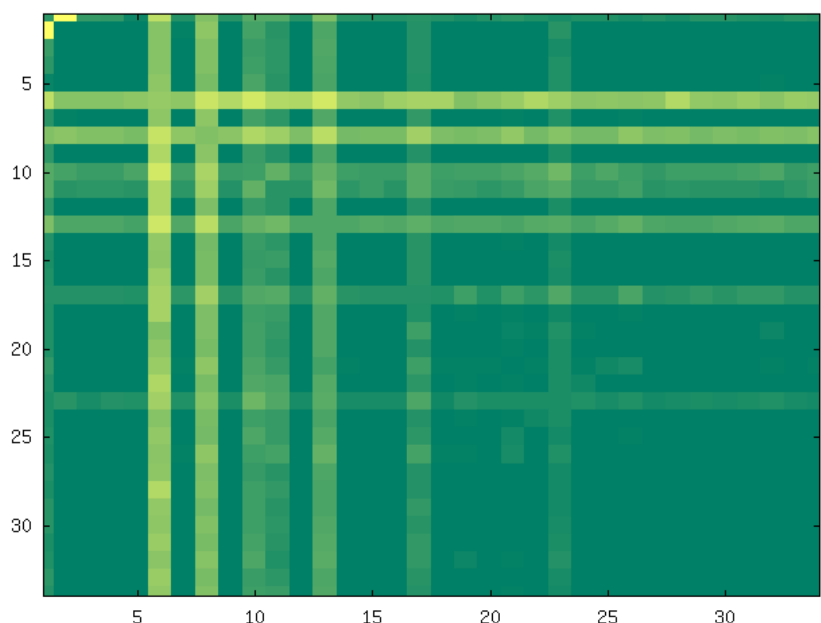
Ionosphere SVD Feature Colormap (Lighter = higher accuracy)
