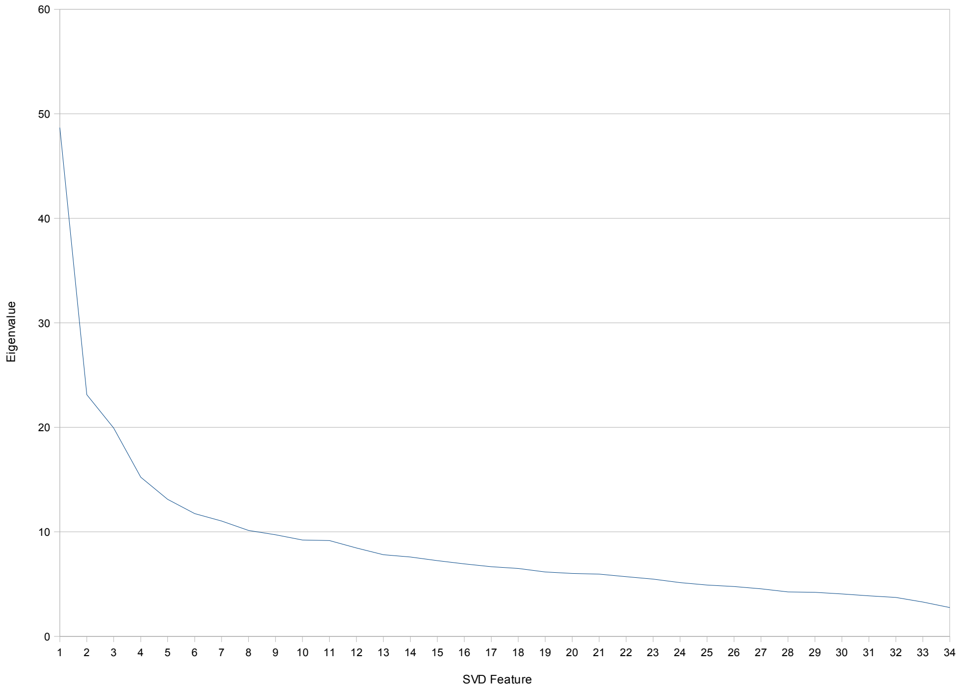
Ionosphere Scree Plot
