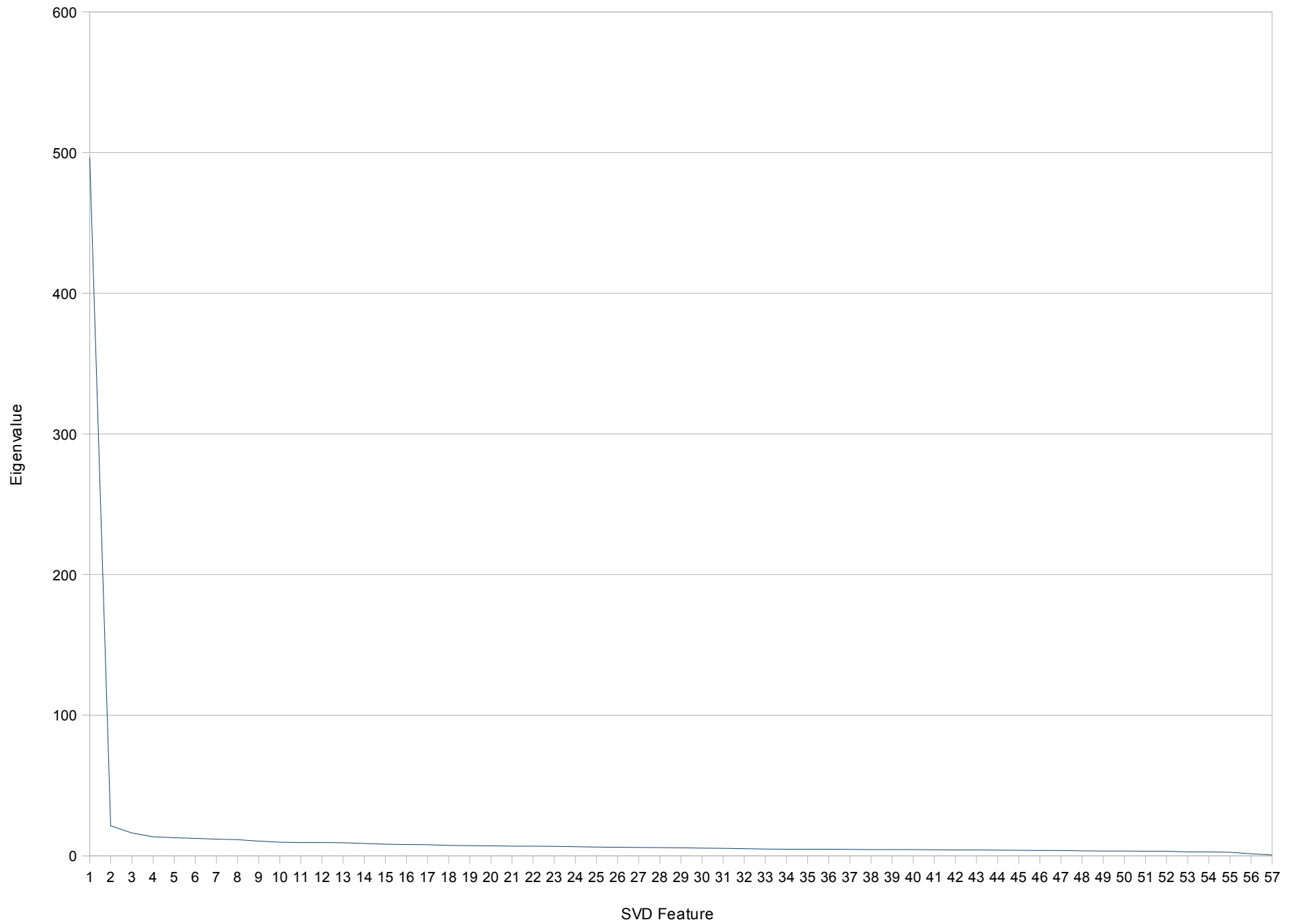
Spam Scree Plot
