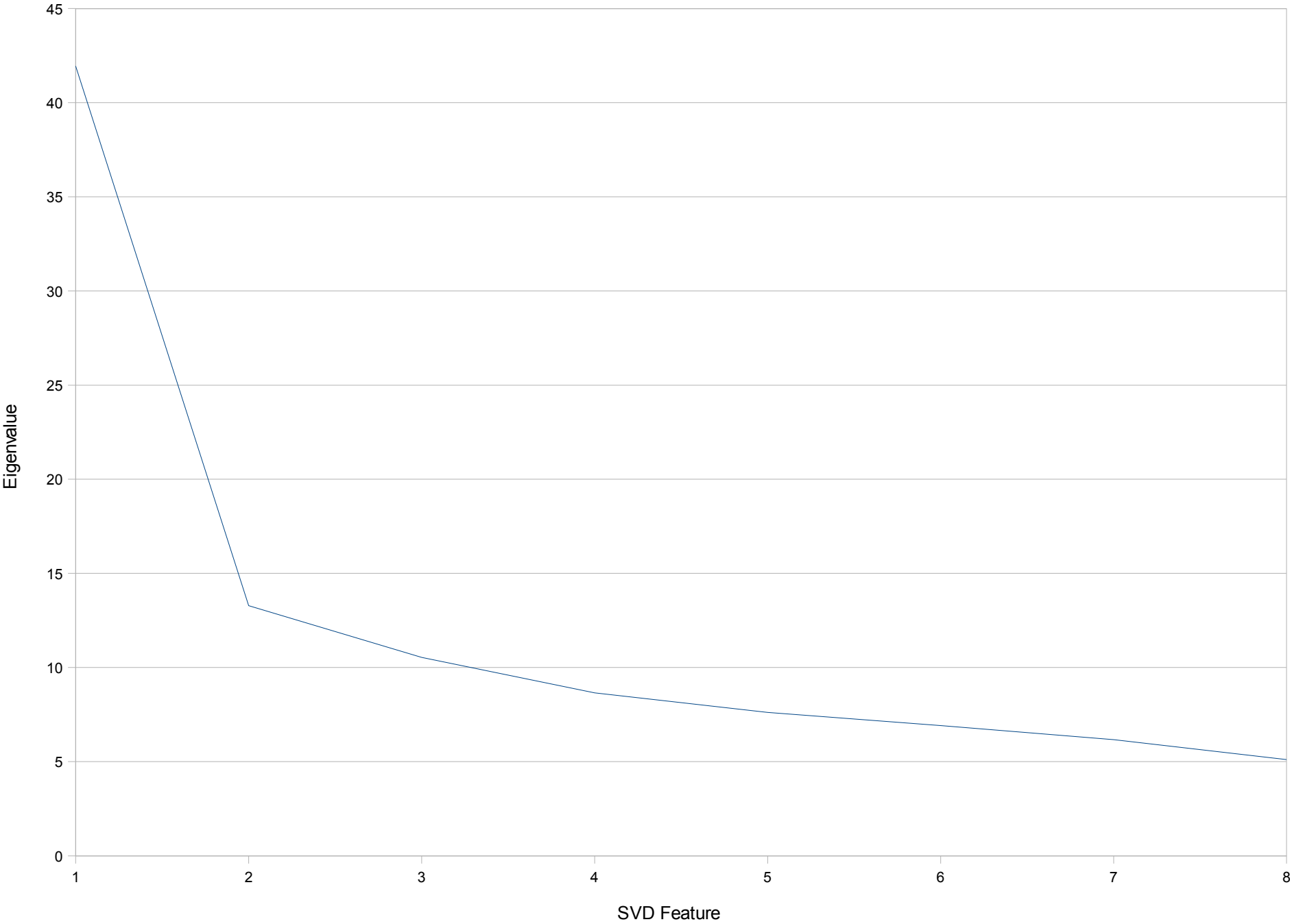
Diabetes Scree Plot
