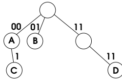
Fig. 2. Multibit trie with stride length of 2.
