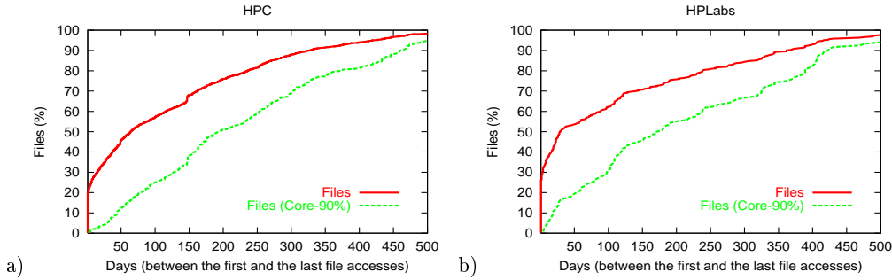
Figure 12: Days between the first and the last file accesses.
