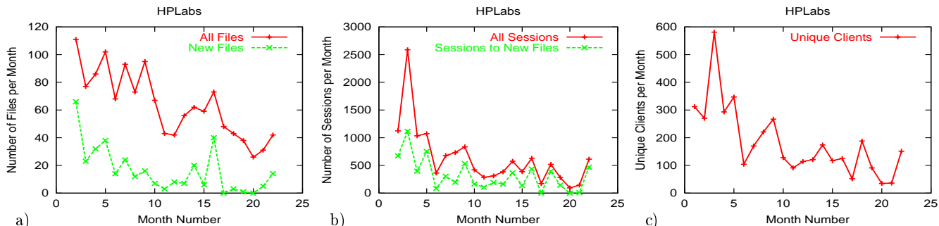
Figure 11: HPLabs workload: a) all and new files, b) all sessions and sessions to new files, c) unique clients.
