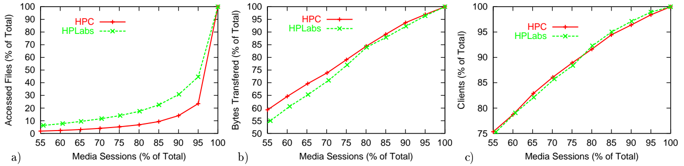
Figure 5: Two workloads compared: a) file set locality, b) bytes-transferred locality c) client set locality.
