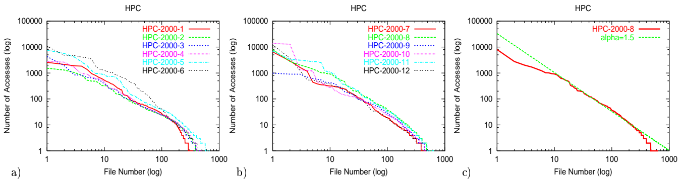
Figure 8: File popularity distribution for HPC workload a) monthly periods, 1st to 6th months b) monthly periods, 7th to 12th months c) 8th month with corresponding Zipf-like function fitting.
