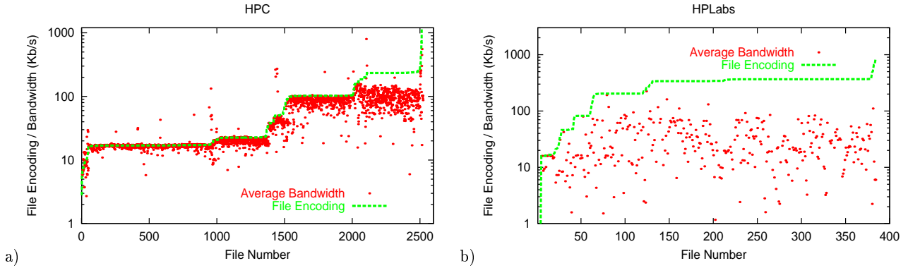
Figure 4: File encoding rates and average available bandwidth of client sessions to those files for both workloads.
