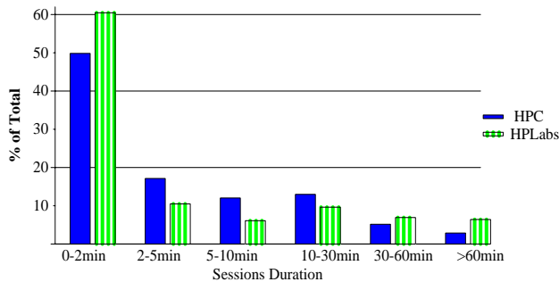
Figure 3: Session duration characterization.
