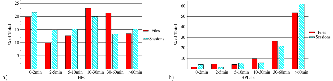
Figure 2: Six classes of file durations and percentage of client sessions to those files: a) HPC and b) HPLabs.
