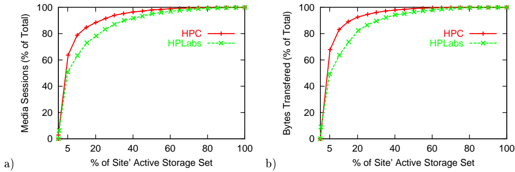
Figure 6: Two workloads compared: storage-set locality and bytes-transferred-storage locality.
