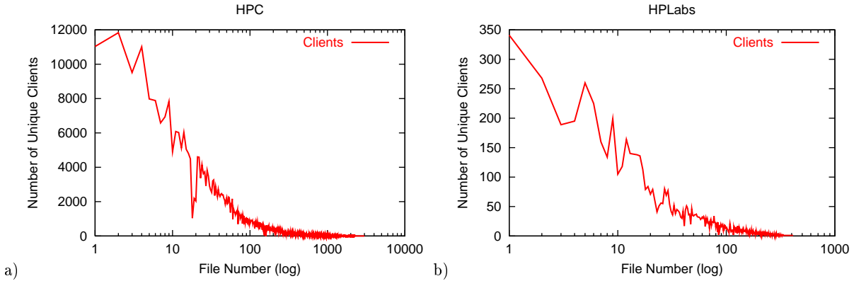
Figure 9: Files sharing statistics: a) HPC and b) HPLabs.
