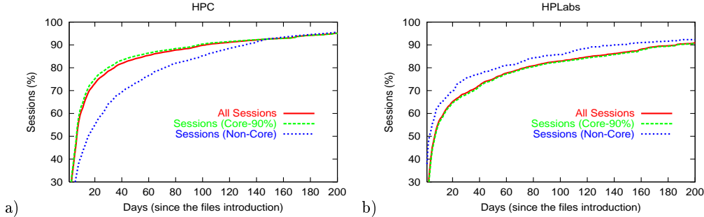
Figure 13: Percent of sessions on days between the first and the last file accesses.
