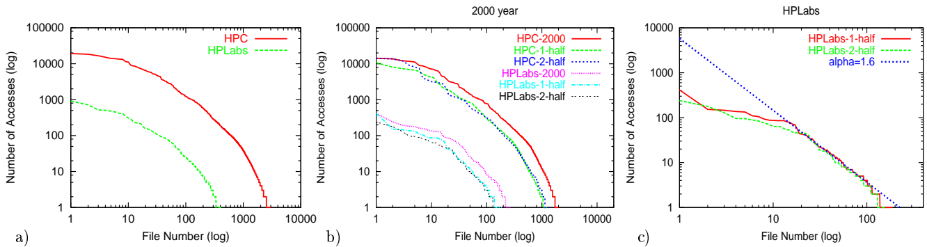
Figure 7: File popularity distribution for both workloads a) over entire duration of the logs, b) over 2000 year and corresponding first and second 6 months in 2000, c) HPLabs workload 6-month periods with corresponding Zipf-like function fitting.
