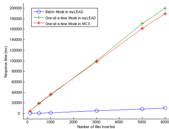
Figure 5. File objects insertion. Response time for iterative and bulk inserts using myLEAD, and in comparison to MCS.
