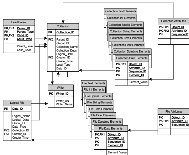
Figure 1. Relational schema of myLEAD database. Many of the organizational details (experiments, projects, etc.) and application specific details (meteorology attributes for instance) are coded in the data for portability of the schema to other domains.
