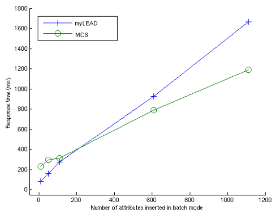
Figure 11. Comparison of bulk adding of attributes in myLEAD and MCS.
