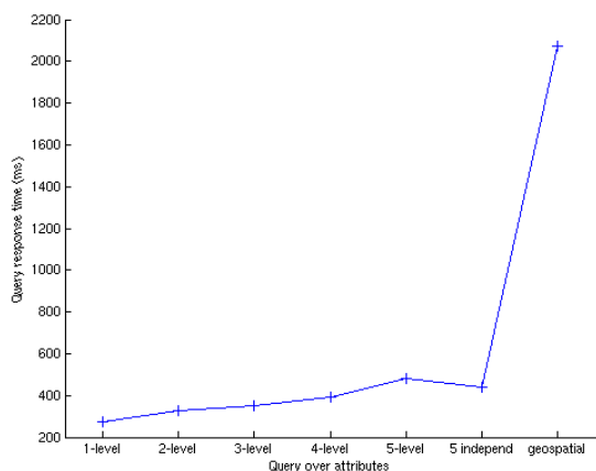
Figure 7. Query over attributes.
