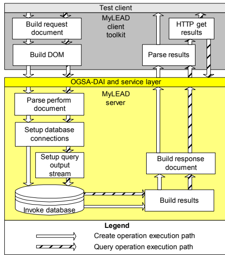
Figure 3. Test framework showing functional decomposition through client toolkit and myLEAD server.
