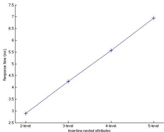
Figure 6. Inserting attributes of increasing levels of nesting. Measures average response time for inserting single nested attribute.
