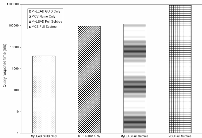
Figure 12. Comparison for two containment queries. The two bars on the left show response time for myLEAD and MCS when experiment IDs are returned. The two bars on the right show response time when the entire subtree of each qualifying experiment is returned.
