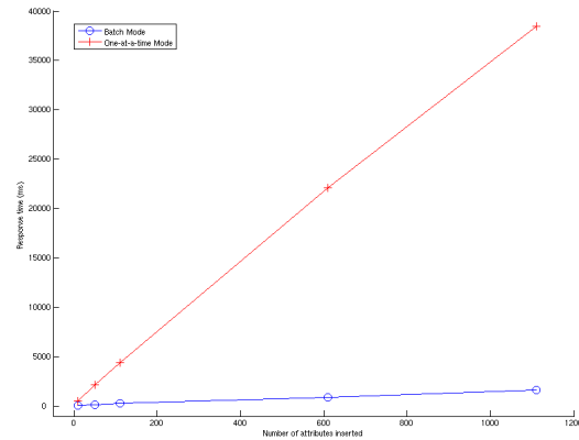
Figure 4. Attribute object insertion. Response time for iterative and bulk inserts.
