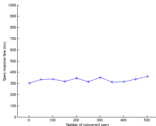
Figure 8. Scalability in number of concurrent users.
