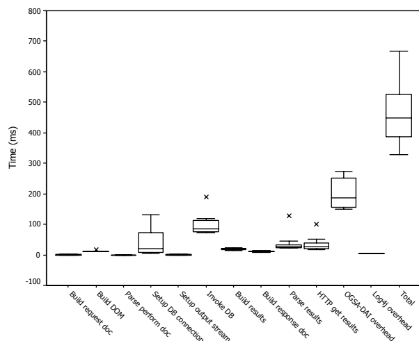
Figure 10. Query collection given a name and return a collection-level subtree consisting of the metadata for the collection metadata plus metadata for 1000 file objects.
