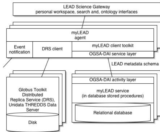
Figure 2. Architecture of myLEAD Personal Workspace.
