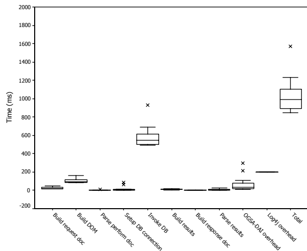
Figure 9. Profile of batch insert of 500 files. Files loaded in bulk are stored to different collections.
