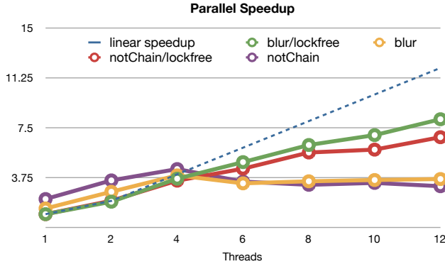
Figure 6. Parallel speedup for the “blur” and “notChain” benchmarks. Speedup is normalized to the sequential times for the lock-free versions (5.21s and 9.83s, respectively). The normalized speedups are remarkably consistent for the lock-free version between the two benchmarks. But the relationship to the original, purely functional version is quite different: at 12 cores, the lock-free LVish version of “blur” is 202\times faster than the original, while “notChain” is only 1.6\times faster, not gaining anything from sharing rather than copying stores due to a lack of fan-out in the state graph.
